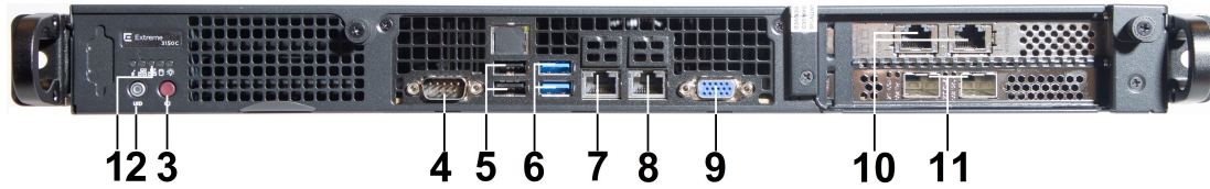
Figure 1: The 3150C Front Panel
